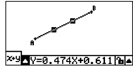
Equation
